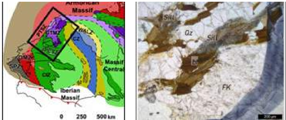
Fig 1. Anatectic complexes in the Central Iberian Zone, a) a simplified structural zone map of the Iberian Massif, b) petrographic image of sillimanite + Fk (PPI).
