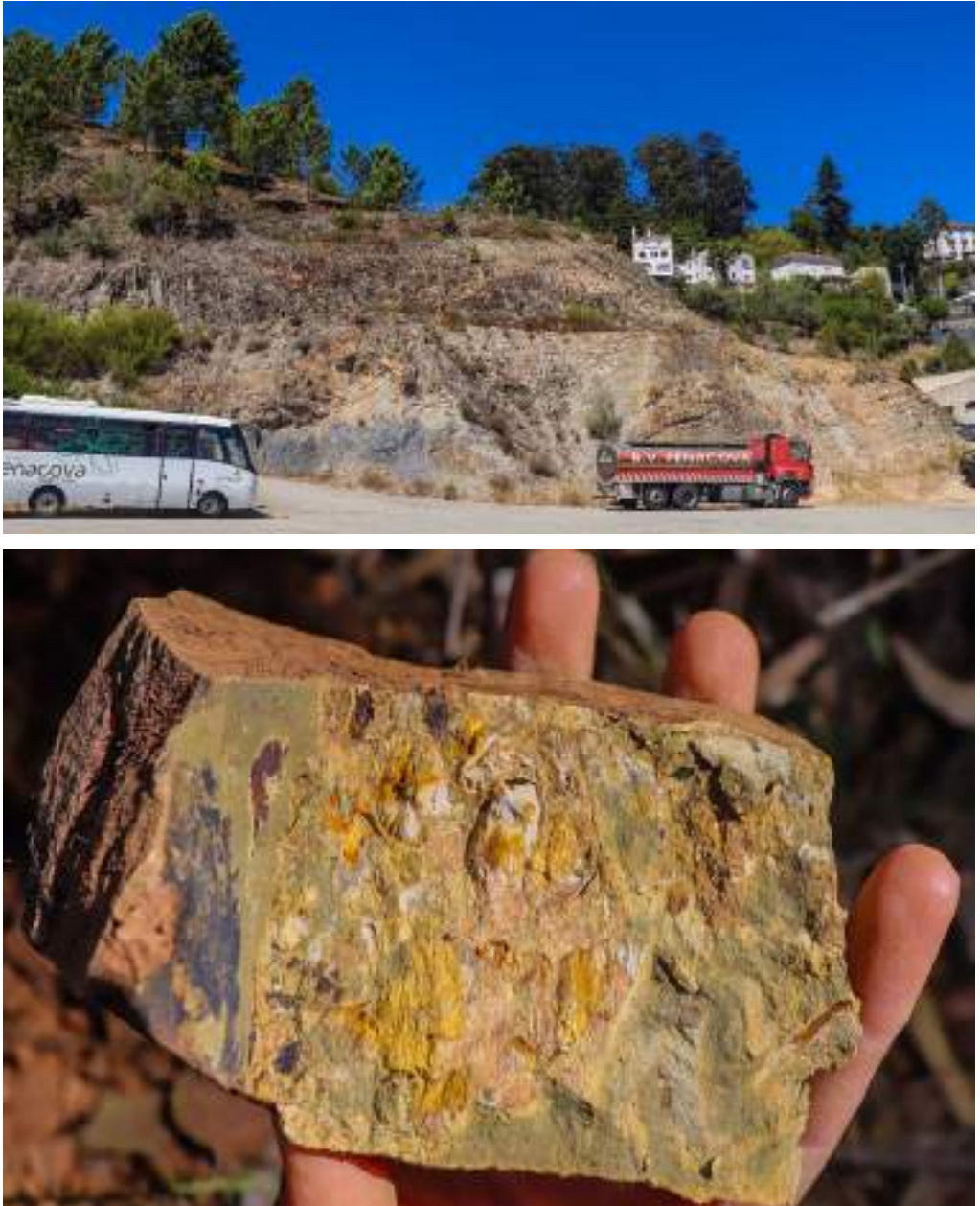
Fig 1. (a) the highly tectonised core of a subsidiary fold in Penacova, with Lower Ordovician quartzites containing lenses of Middle Ordovician mudstones, (b) careful collection of fossil fauna permits a high-resolution stratigraphy, here with an assemblage related to the cold water 'Hirnantia fauna' (Ribeira do Braçal Fm) from immediately below diamictites of the Casal Carvalho Fm.
