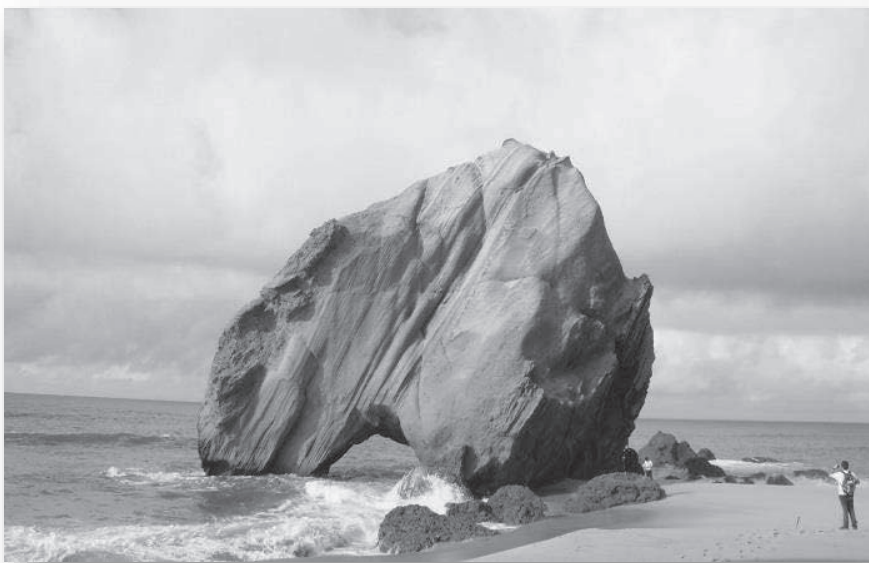
The Guincho rock of Santa Cruz geosite (Lusitanian Basin, Central Portugal) composed of Upper Jurassic coarse siliciclastic sediments infilling a submarine incision channel (from Pena dos Reis and Henriques, 2017).
