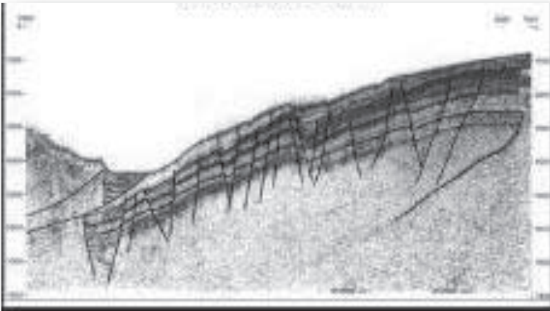
Imbricate faulting over Timor deep-water.
