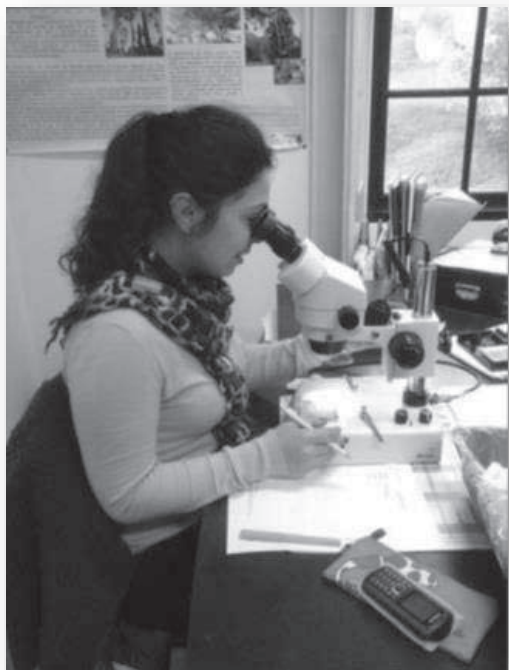
Observation and counting sedimentary charcoals to identify paleo-fire events in the Lower Tagus Valley.
