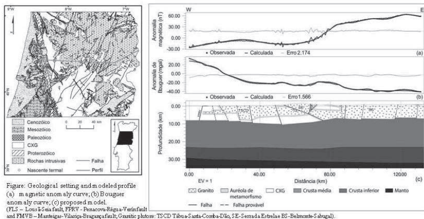
Geological setting and modeled profile (from Machadinho et al., 2017).
