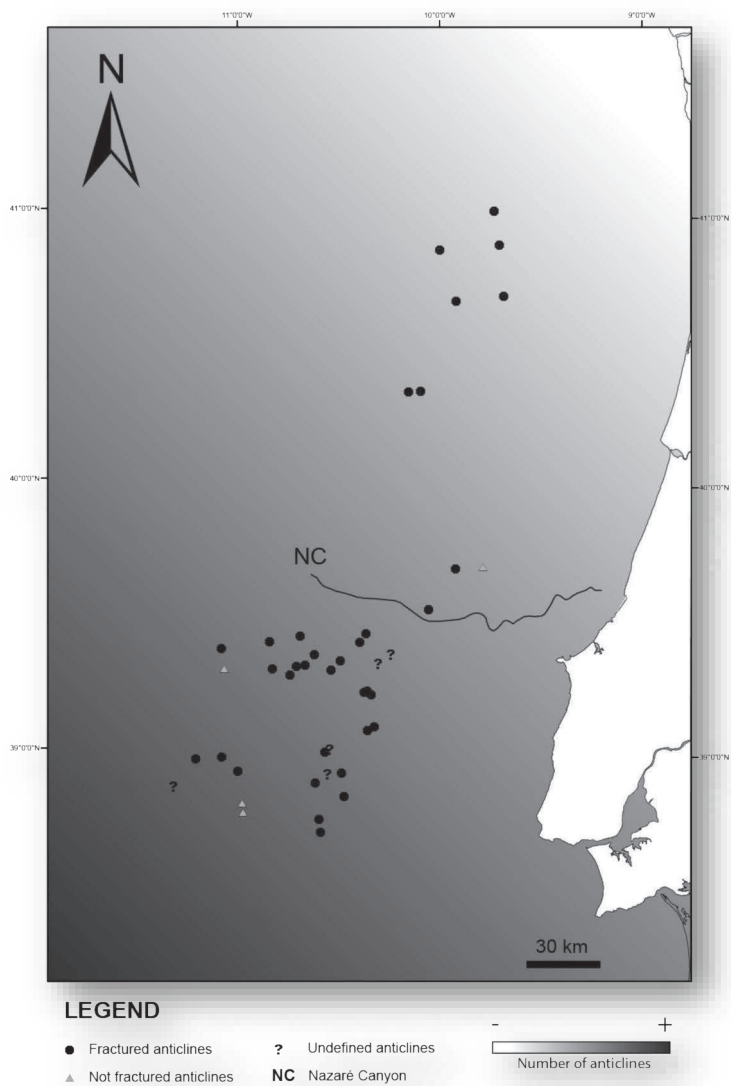
Representation of the deformation spatial variation based on the fractured anticlines distribution (from Reis et al., 2017; in prep.).
